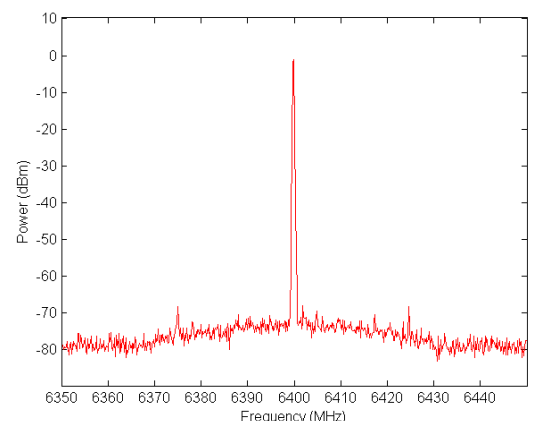
Figure 11a: 6.4GHz Narrow Band Spectrum
